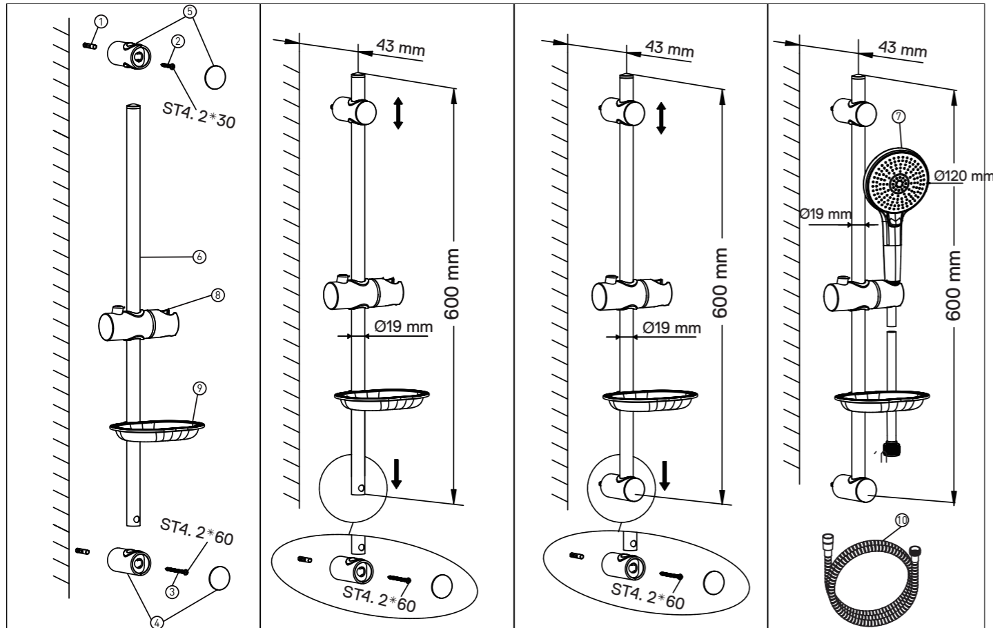
Hand shower set 3- function chromed CIC141
