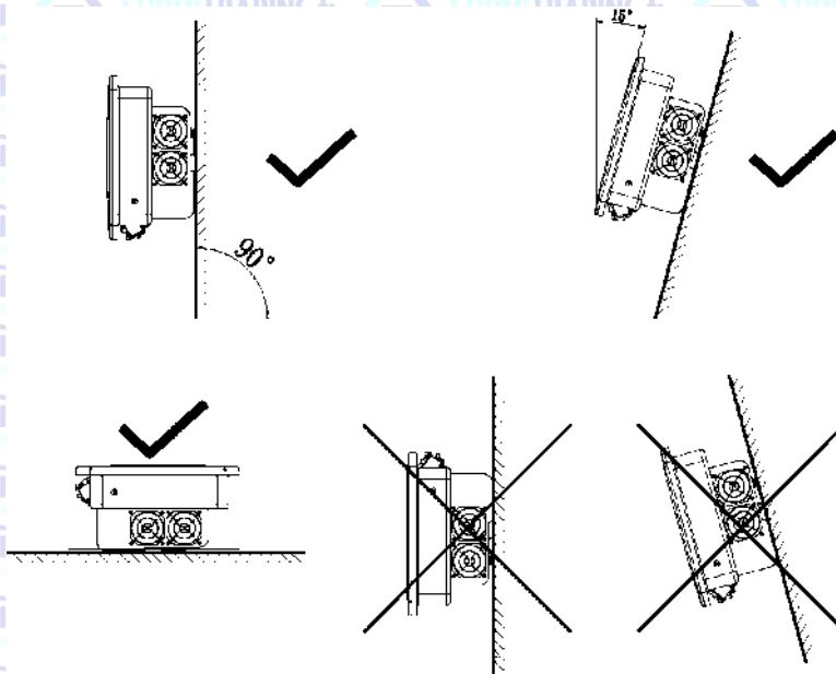
Fig 5.1 Installation diagram
